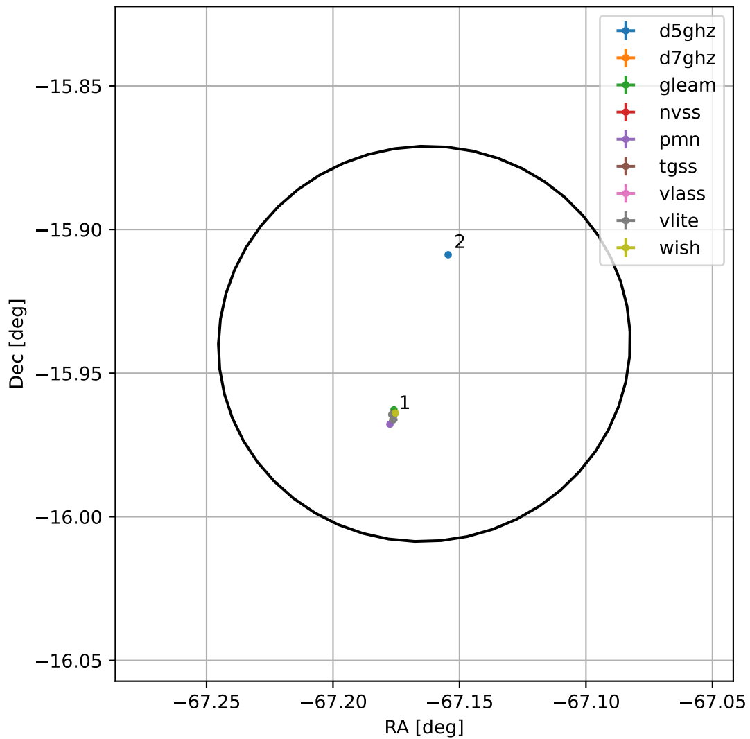
4FGL J1931.3-1556
