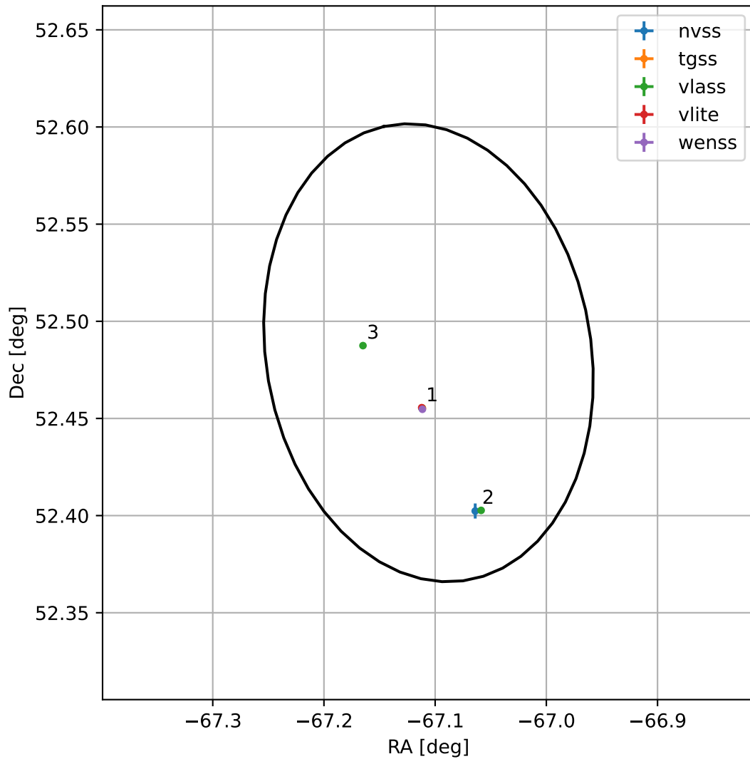
4FGL J1931.5+5229
