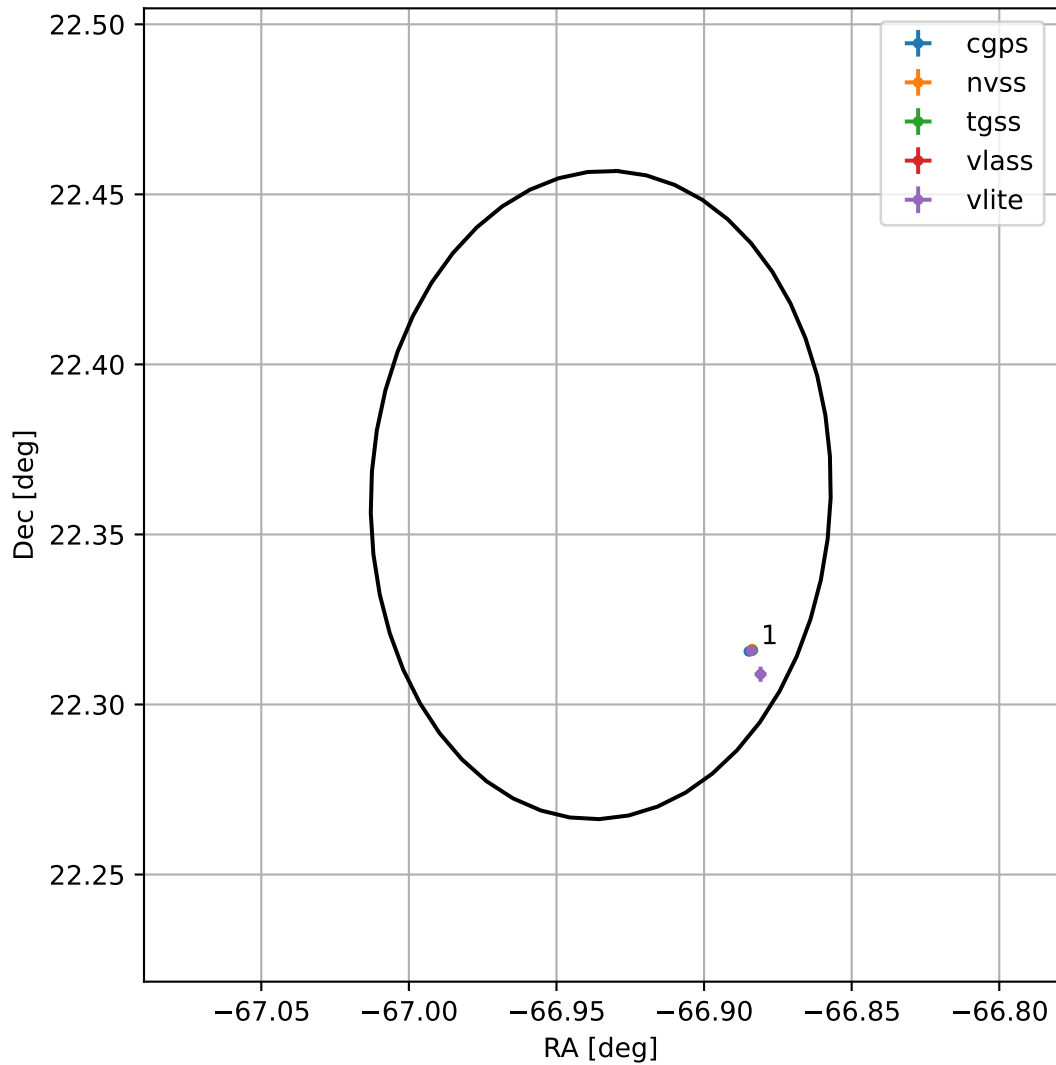
4FGL J1932.2+2221
