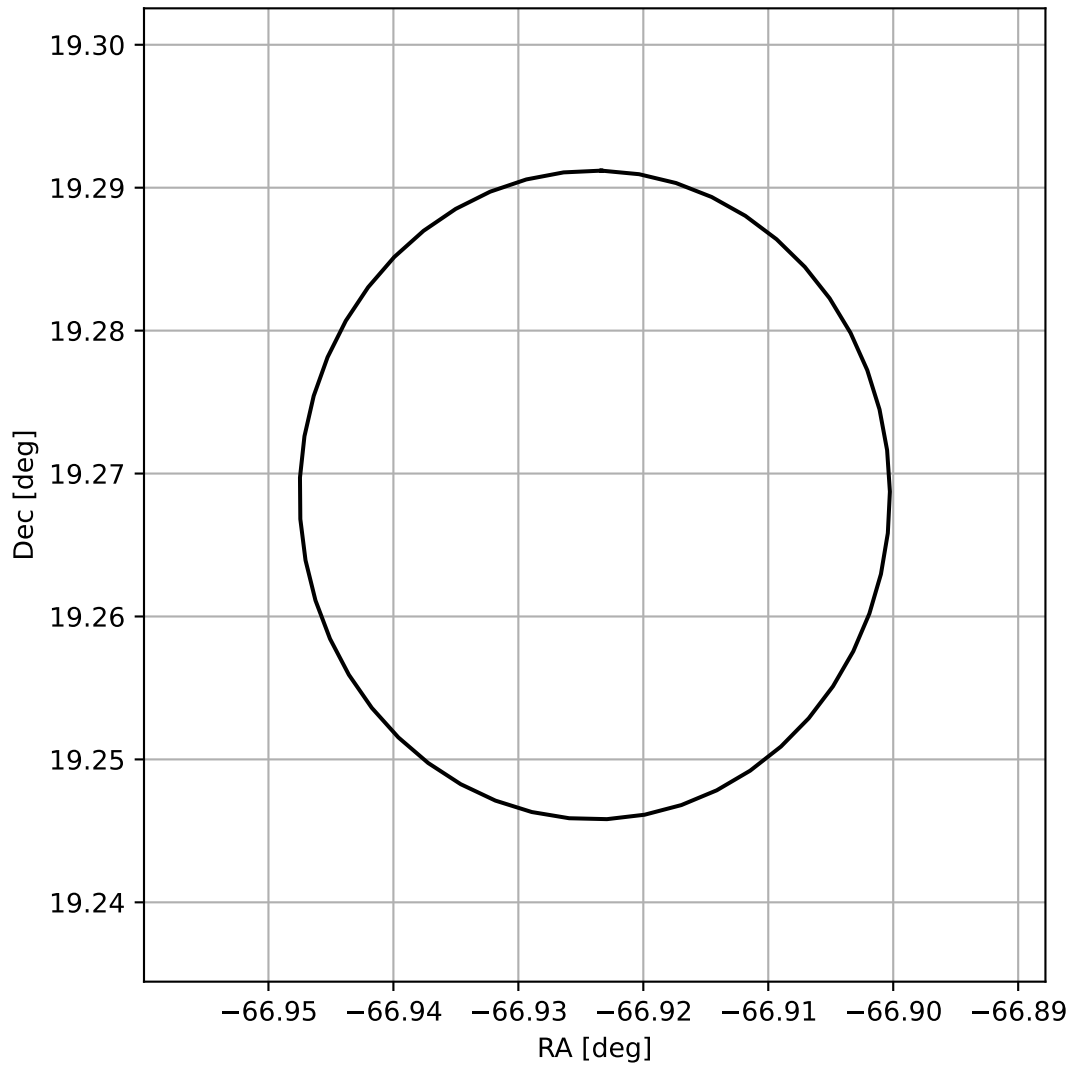
4FGL J1932.3+1916
