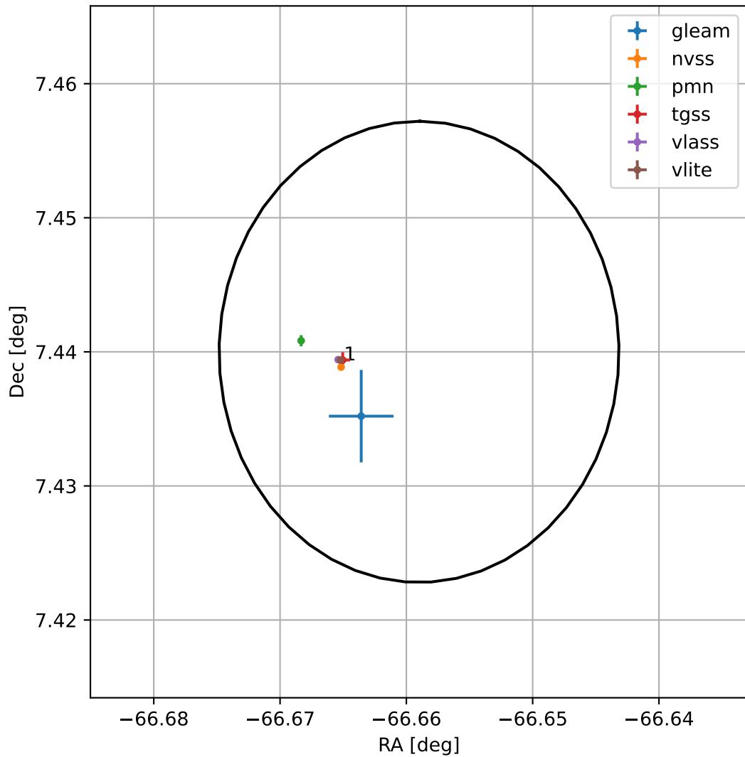
4FGL J1933.3+0726
