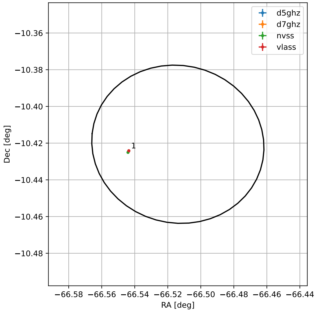
4FGL J1933.9-1025
