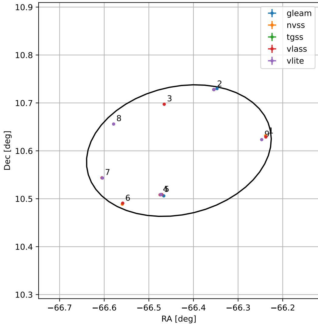
4FGL J1934.2+1036
