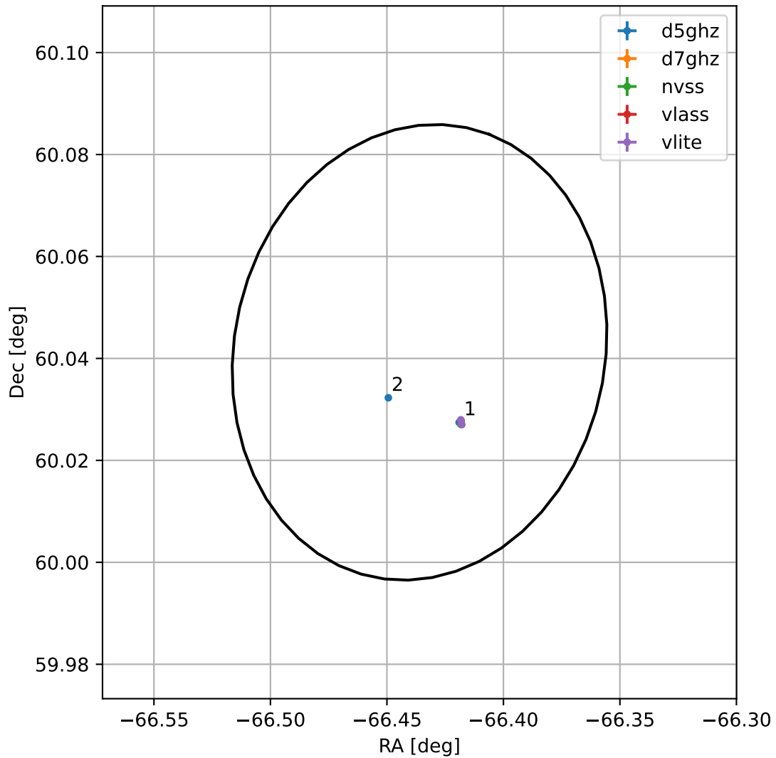
4FGL J1934.2+6002
