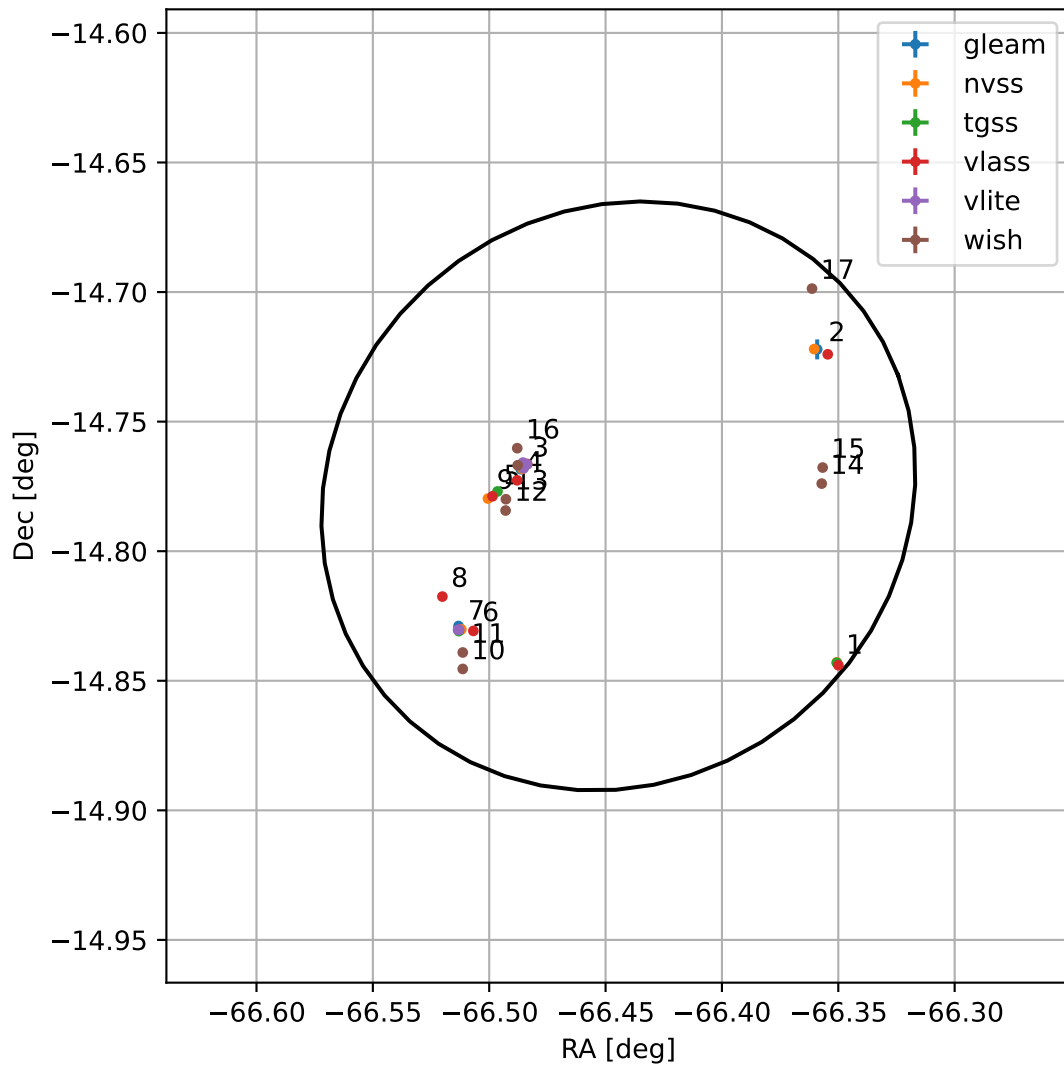
4FGL J1934.2-1446
