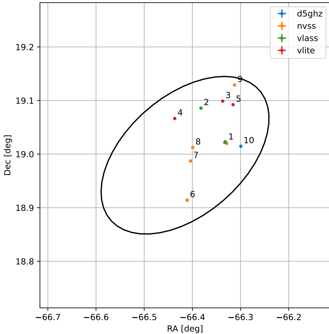
4FGL J1934.3+1859
