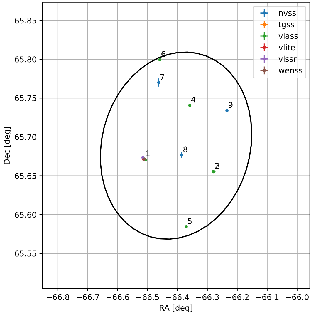
4FGL J1934.3+6541
