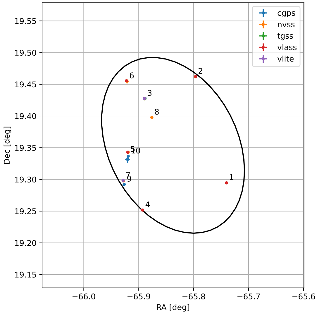
4FGL J1936.6+1921
