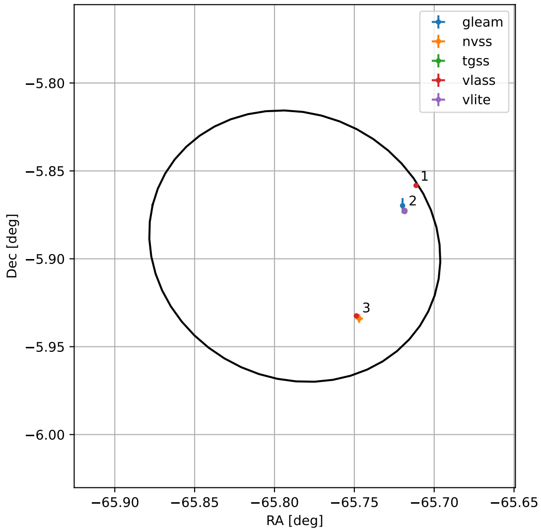
4FGL J1936.8-0553
