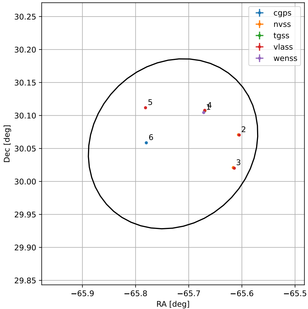
4FGL J1937.0+3003
