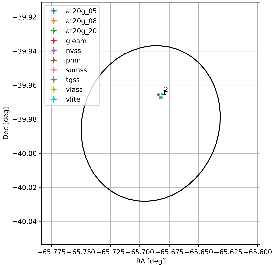
4FGL J1937.2-3958
