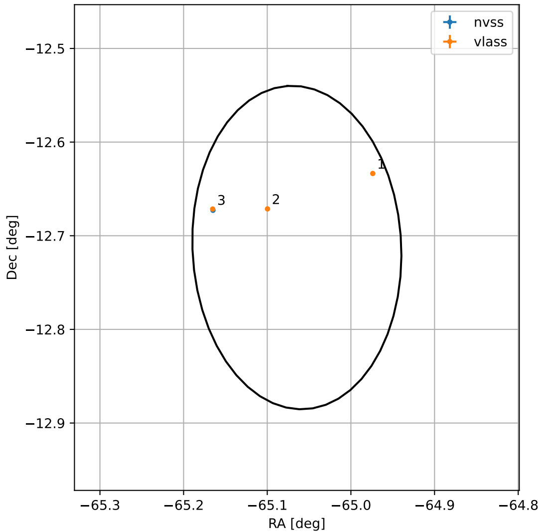
4FGL J1939.7-1242
