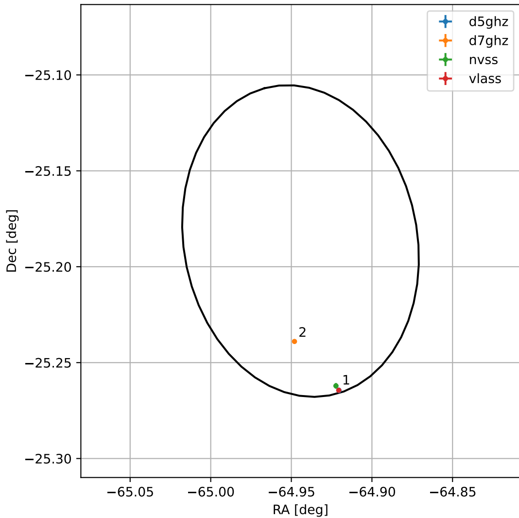
4FGL J1940.2-2511
