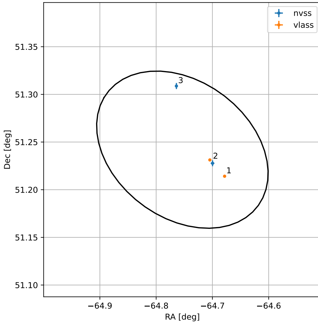
4FGL J1940.9+5114
