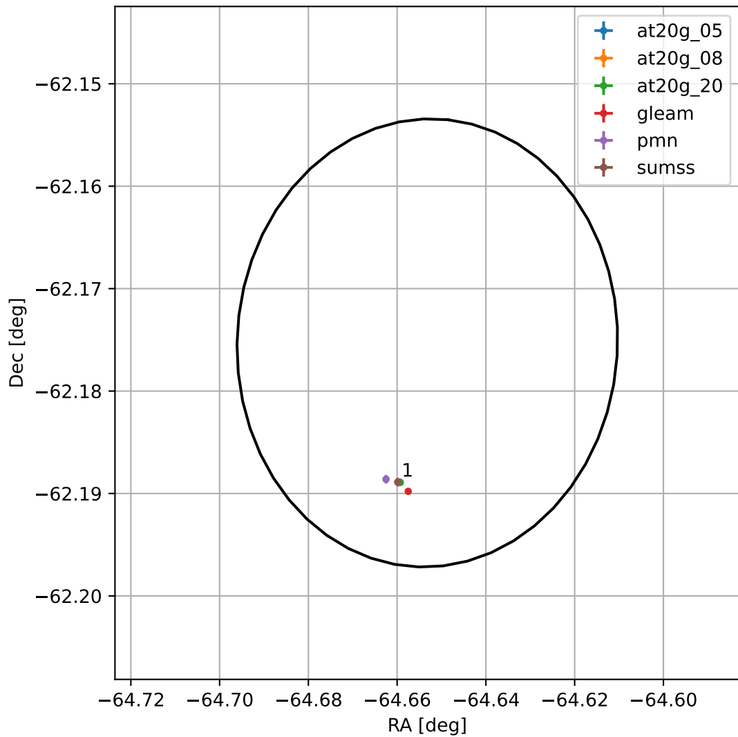
4FGL J1941.3-6210
