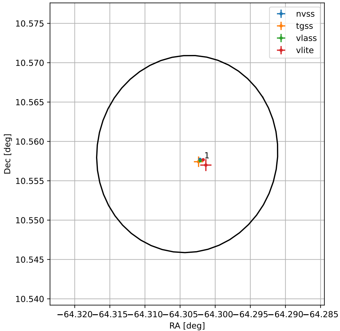
4FGL J1942.7+1033
