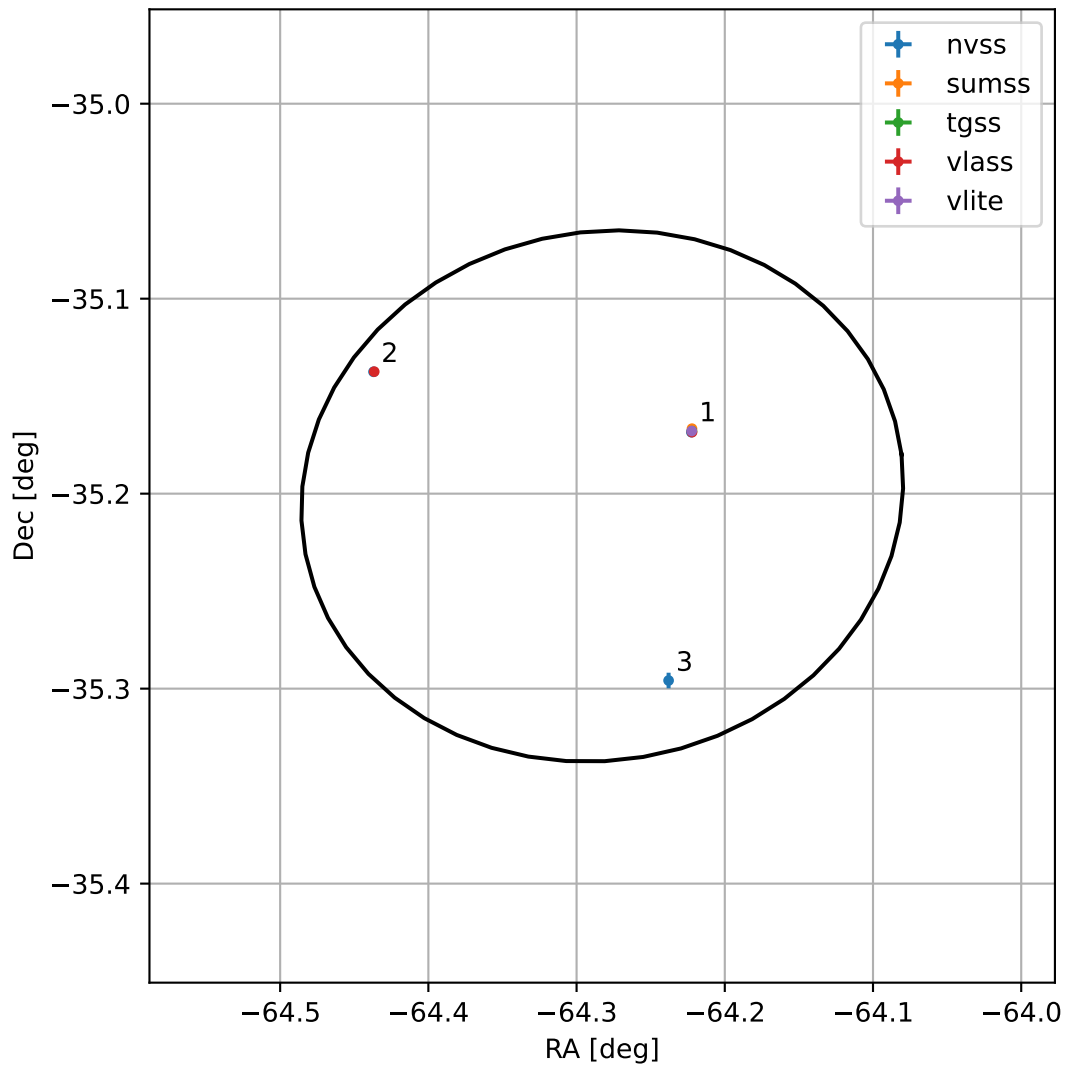
4FGL J1942.8-3512
