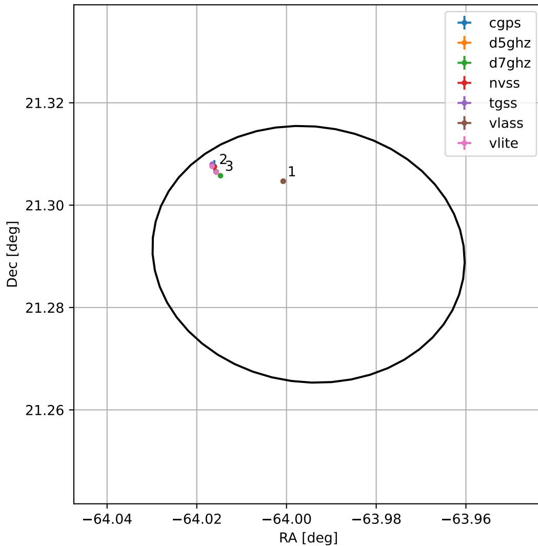
4FGL J1944.0+2117
