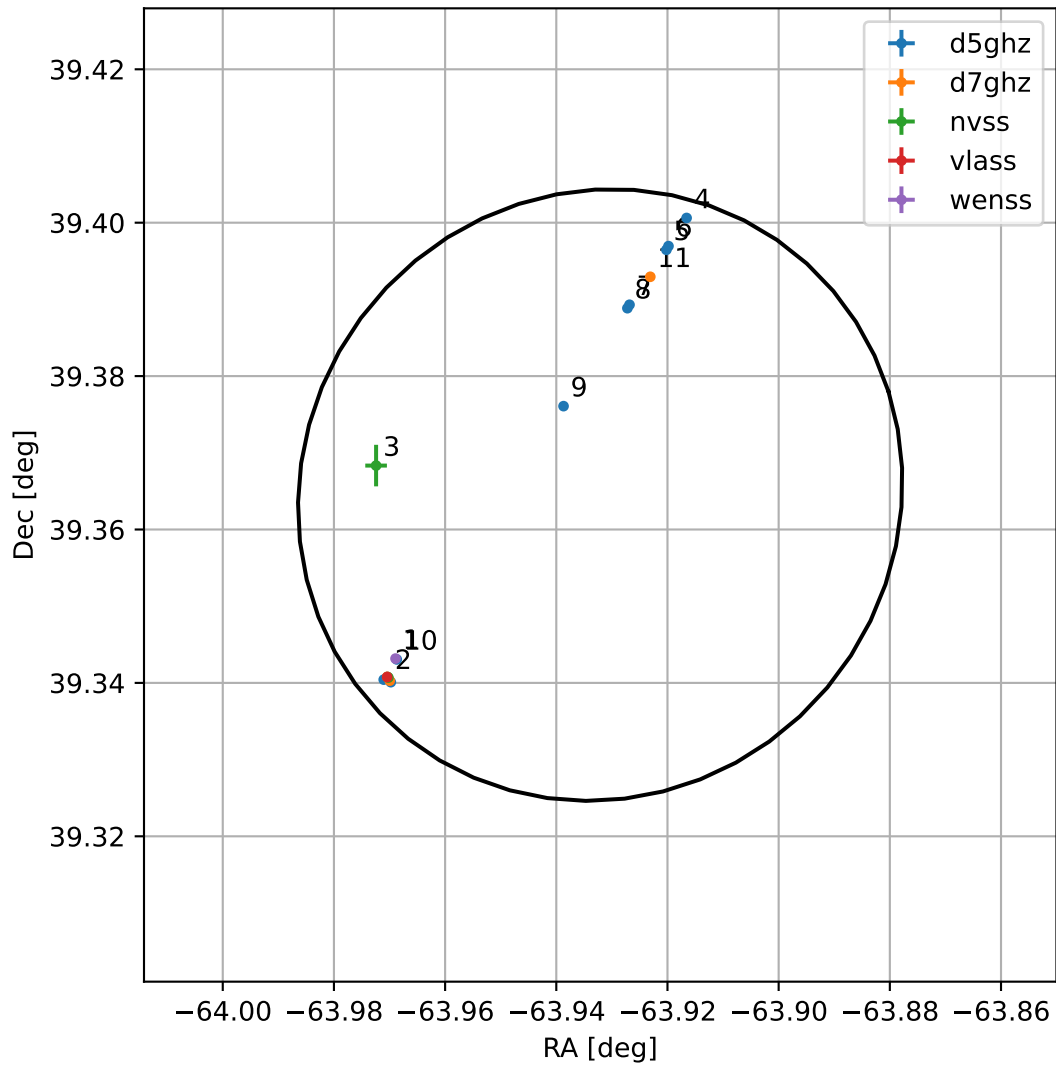
4FGL J1944.2+3921
