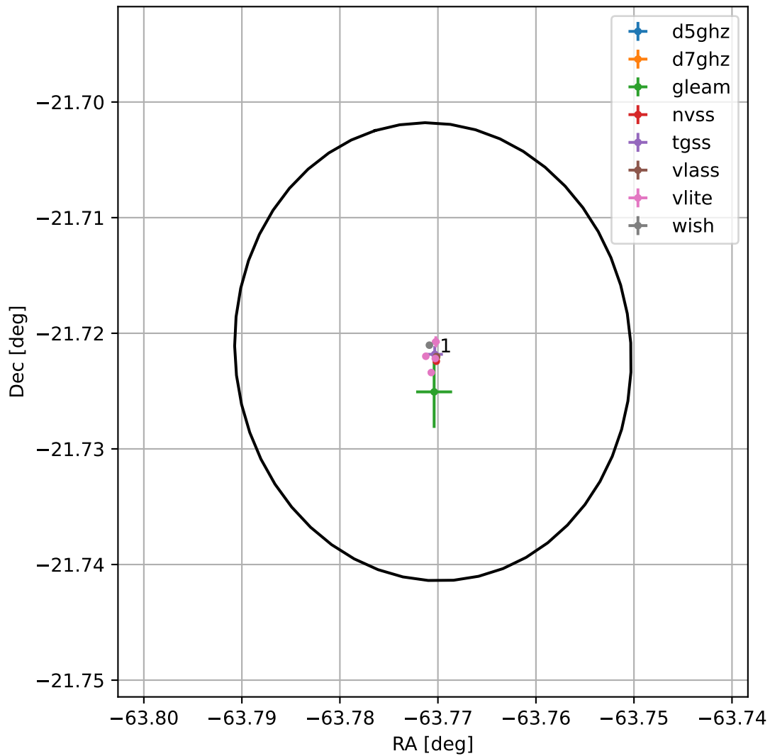
4FGL J1944.9-2143
