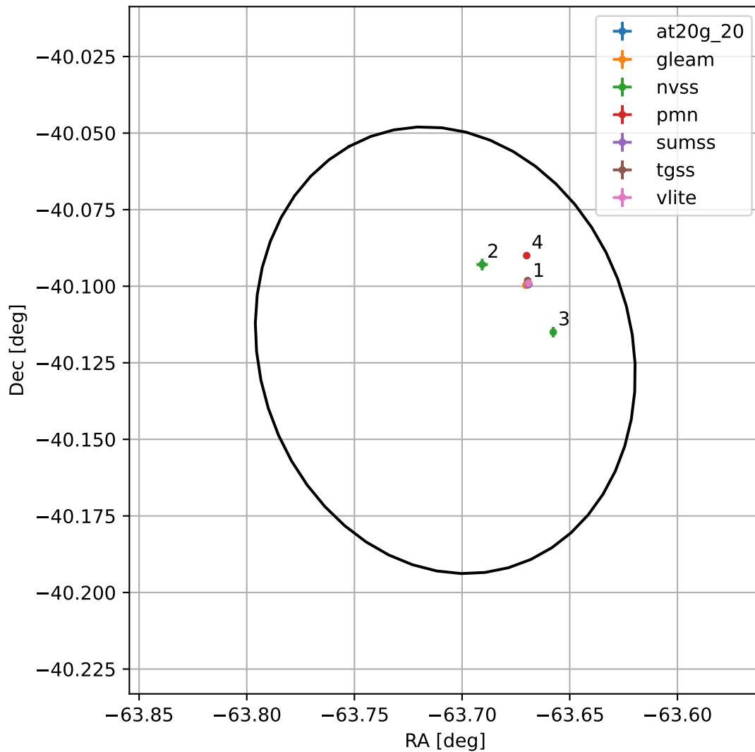
4FGL J1945.1-4007
