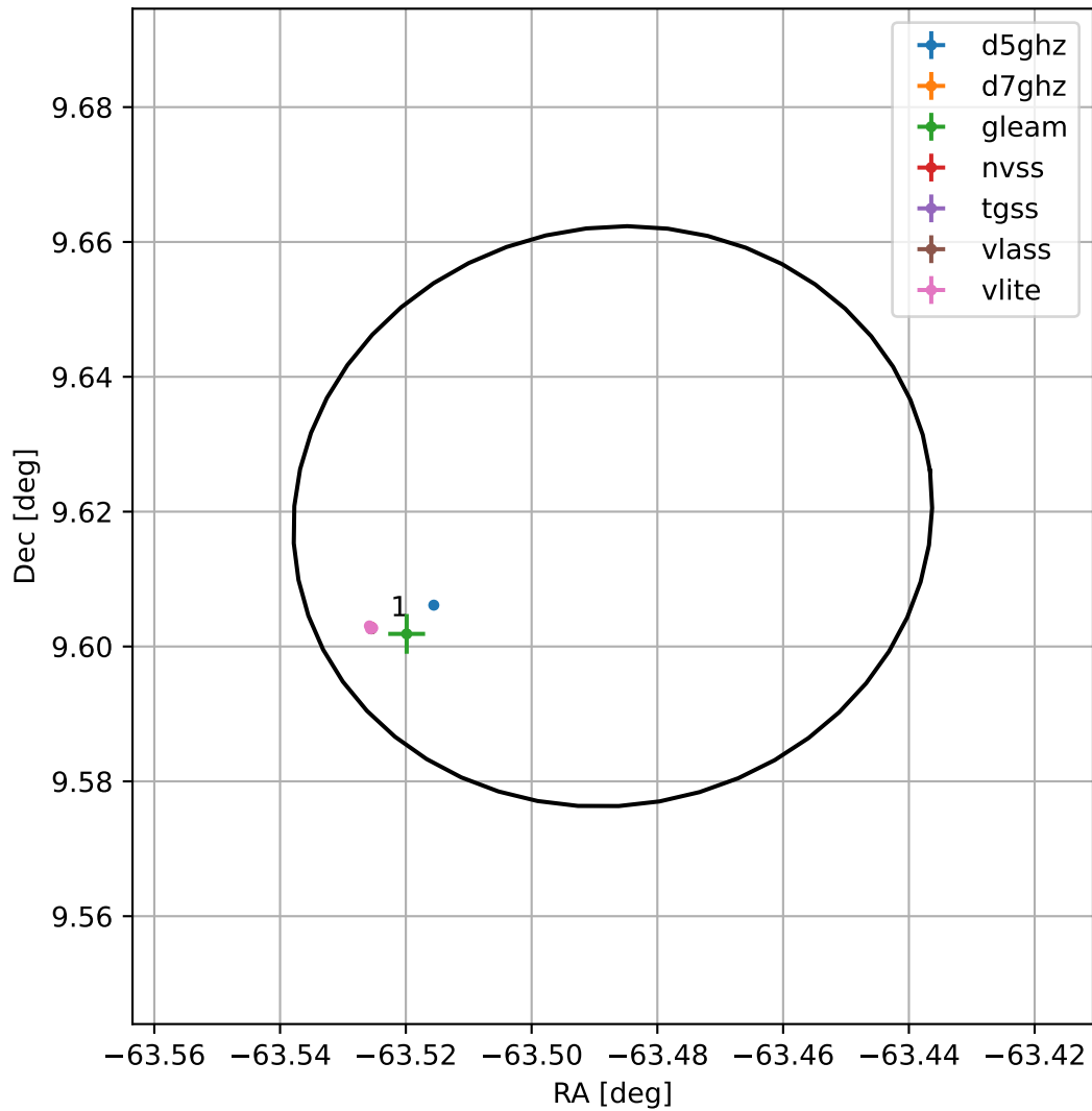
4FGL J1946.0+0937
