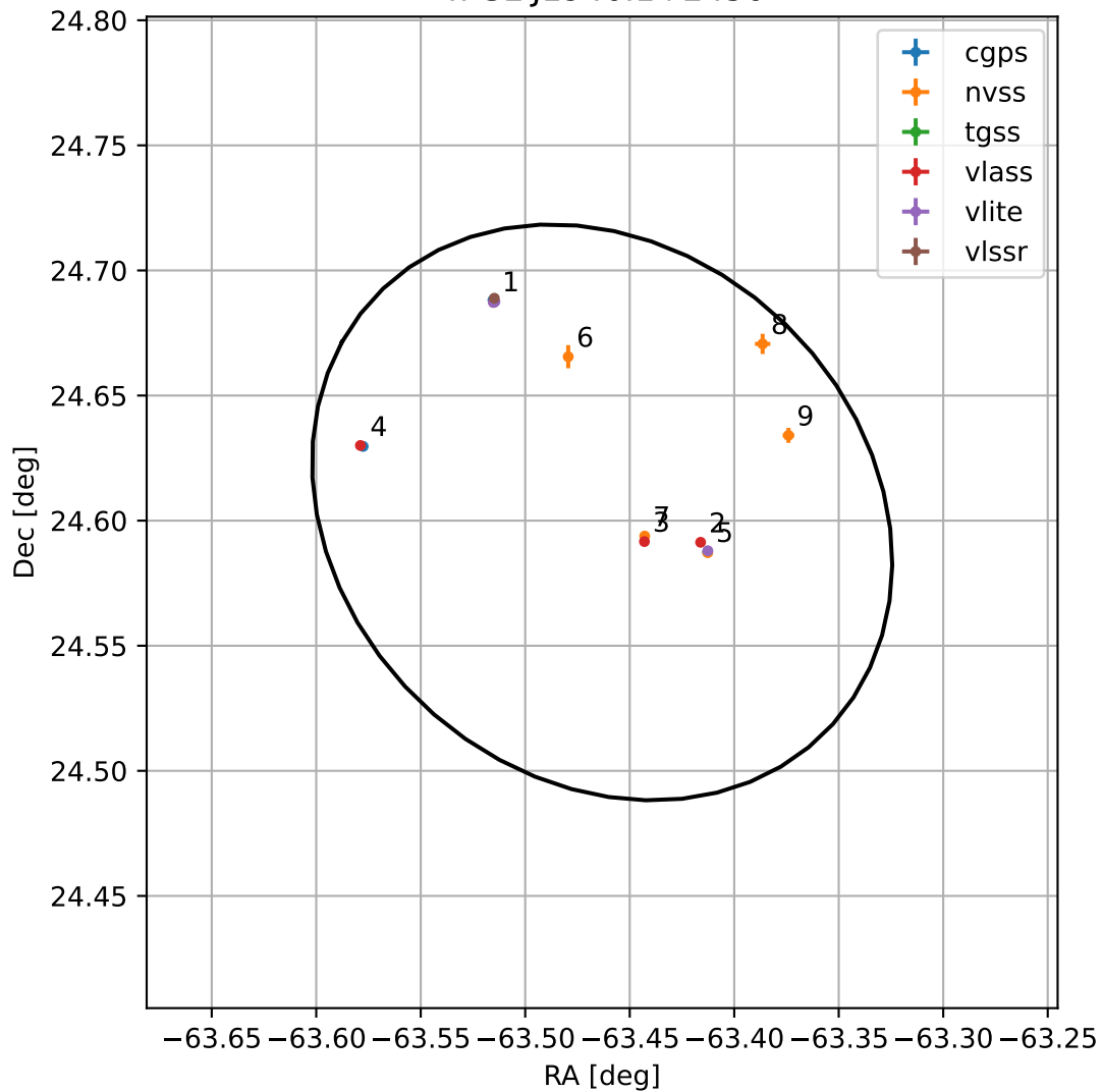
4FGL J1946.1+2436
