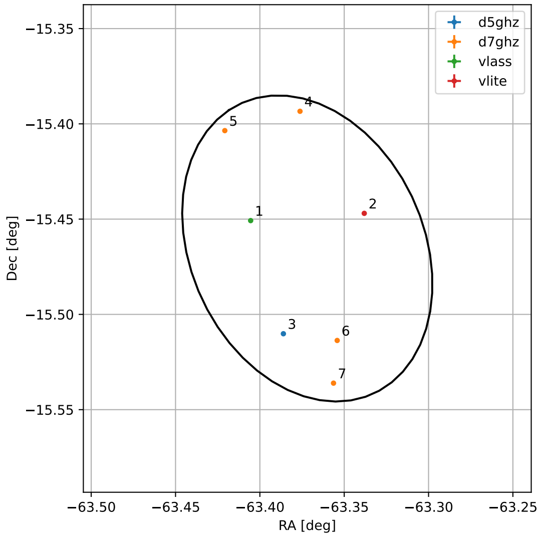
4FGL J1946.5-1527
