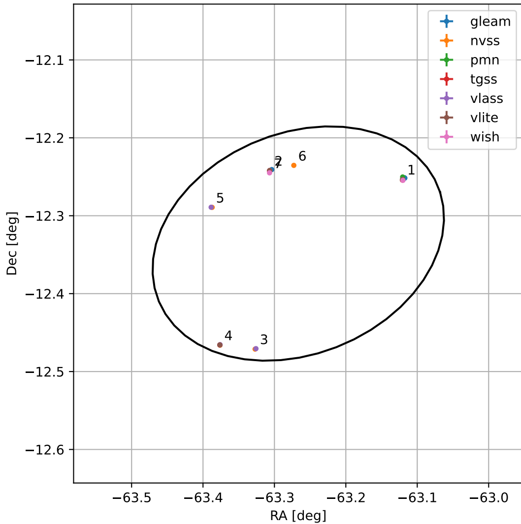
4FGL J1946.9-1220
