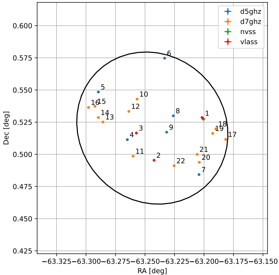
4FGL J1947.0+0031
