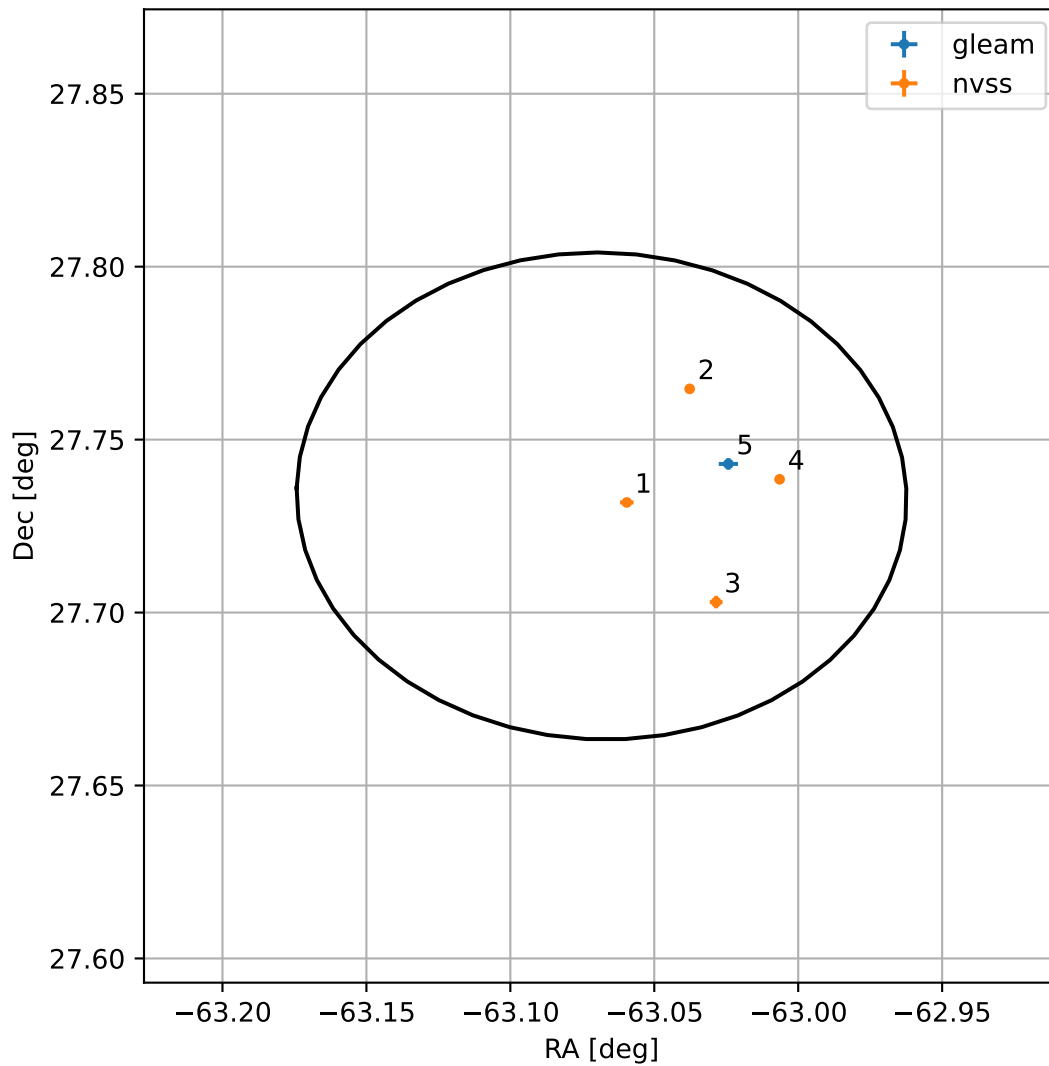
4FGL J1947.7+2744
