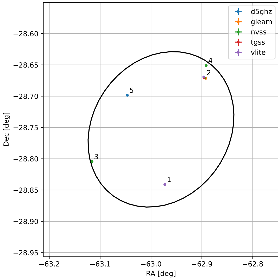
4FGL J1948.0-2845
