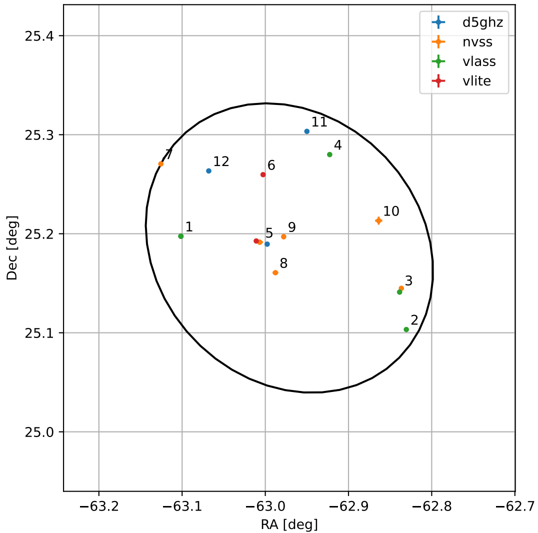
4FGL J1948.1+2511
