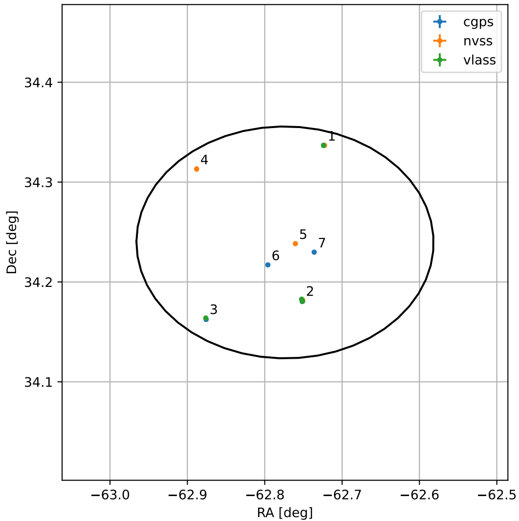
4FGL J1948.9+3414
