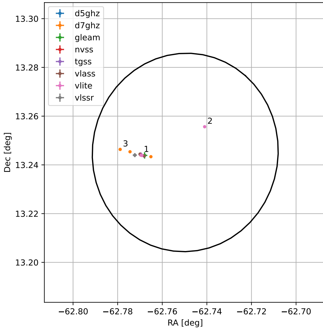
4FGL J1949.0+1314
