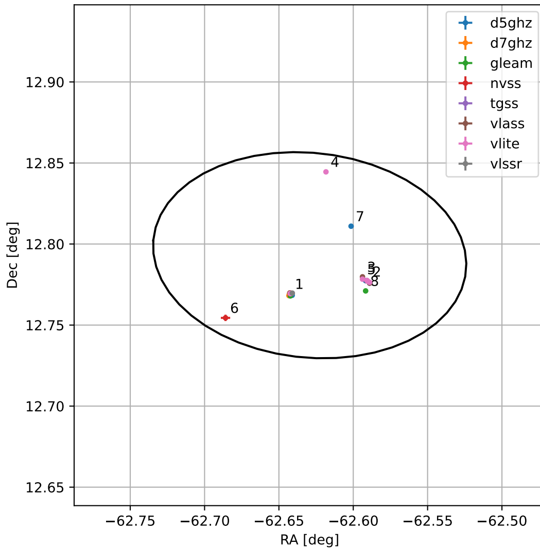
4FGL J1949.4+1247
