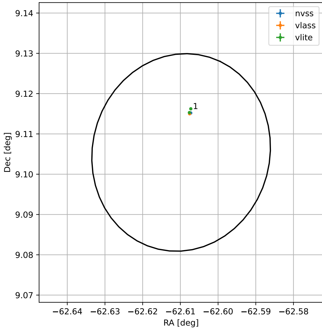
4FGL J1949.5+0906
