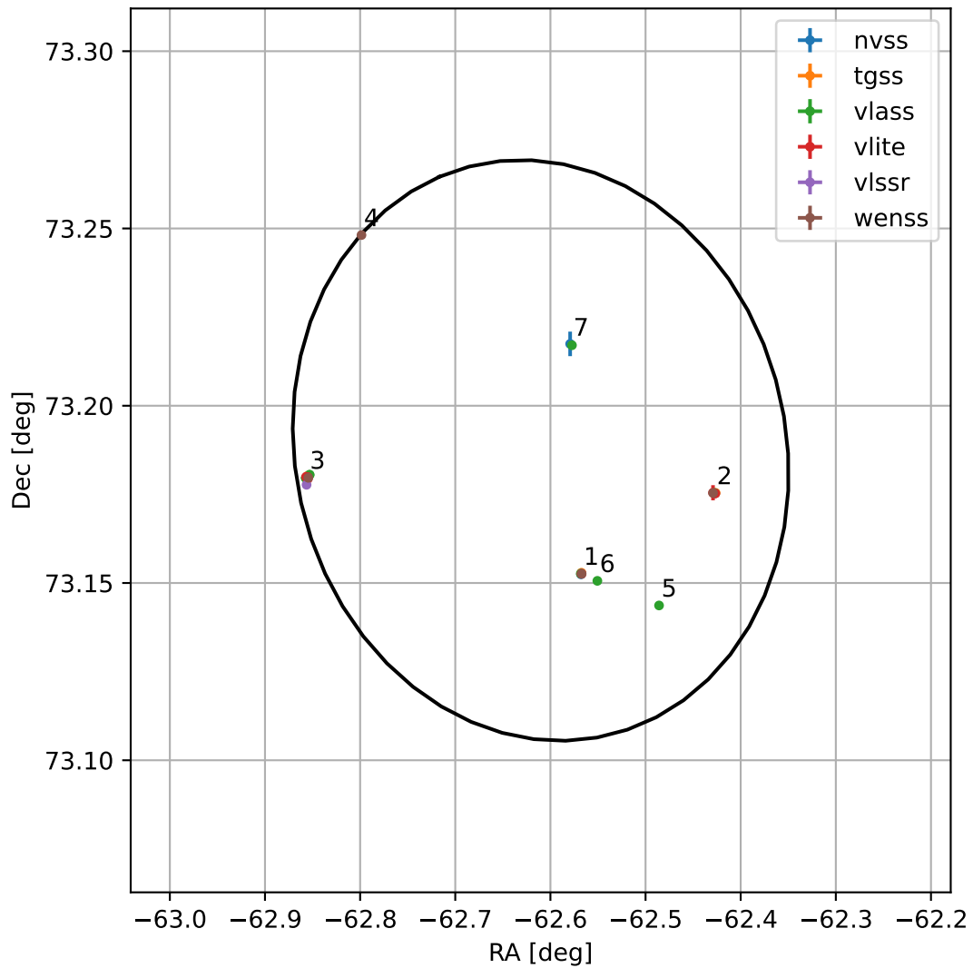
4FGL J1949.5+7311
