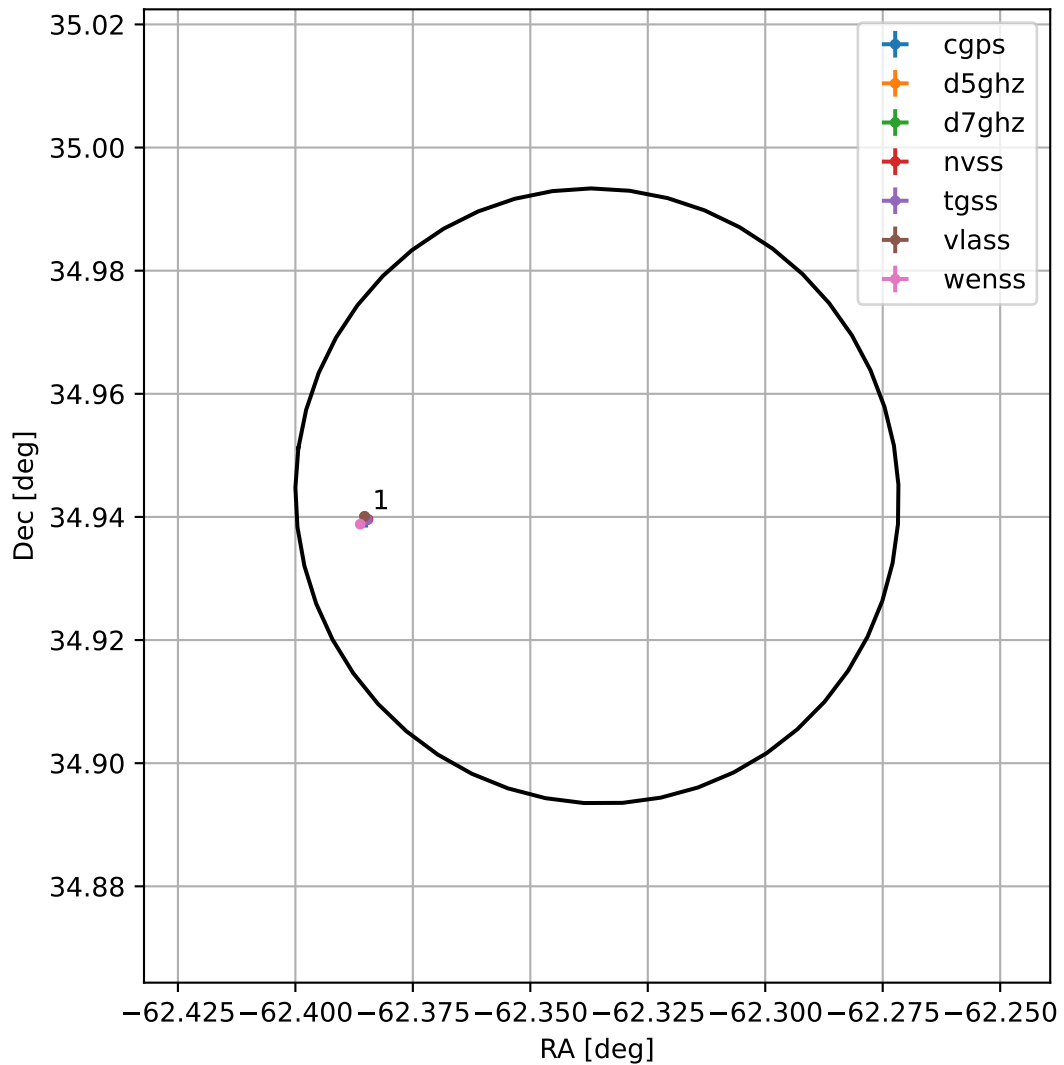
4FGL J1950.6+3456
