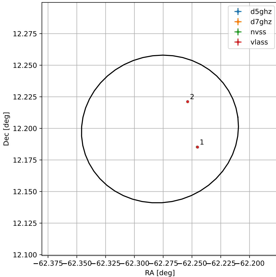
4FGL J1950.8+1211
