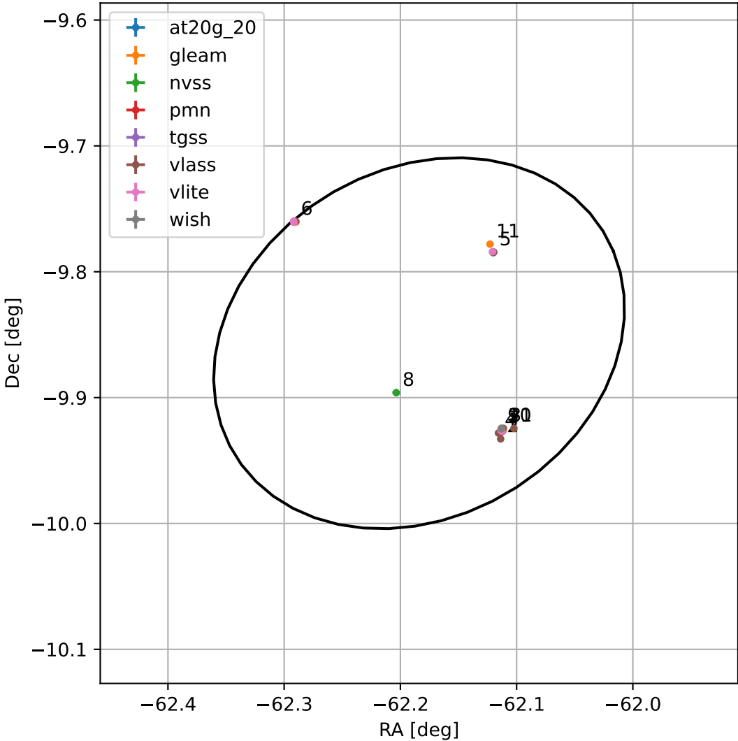
4FGL J1951.2-0951
