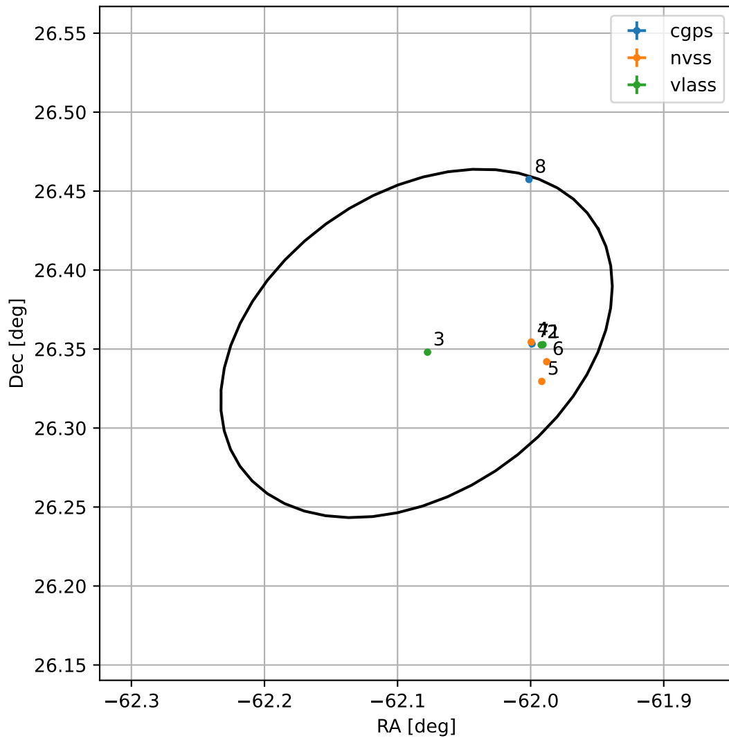
4FGL J1951.6+2621
