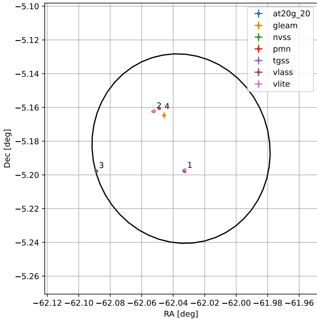
4FGL J1951.8-0511
