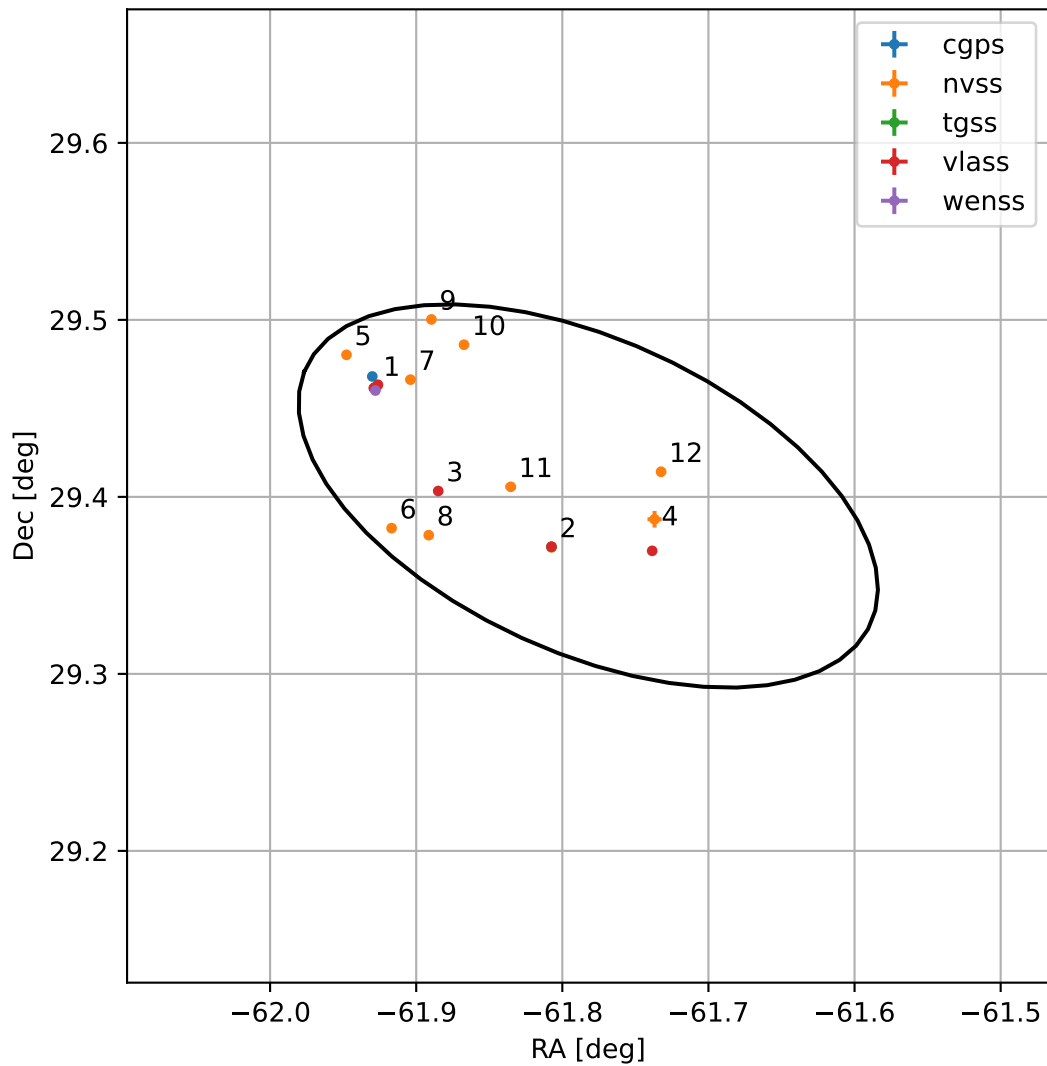
4FGL J1952.8+2924
