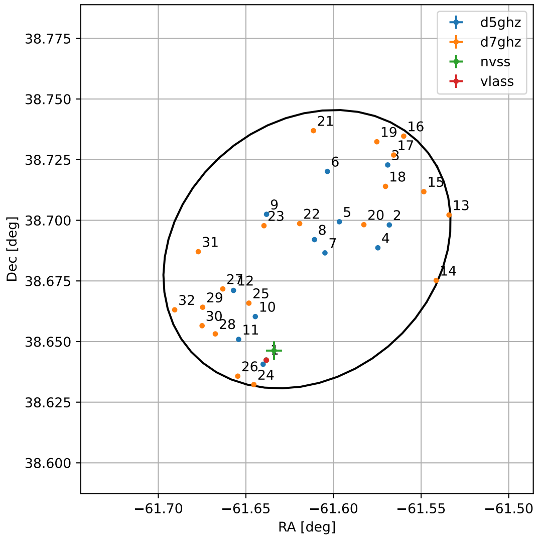
4FGL J1953.5+3841
