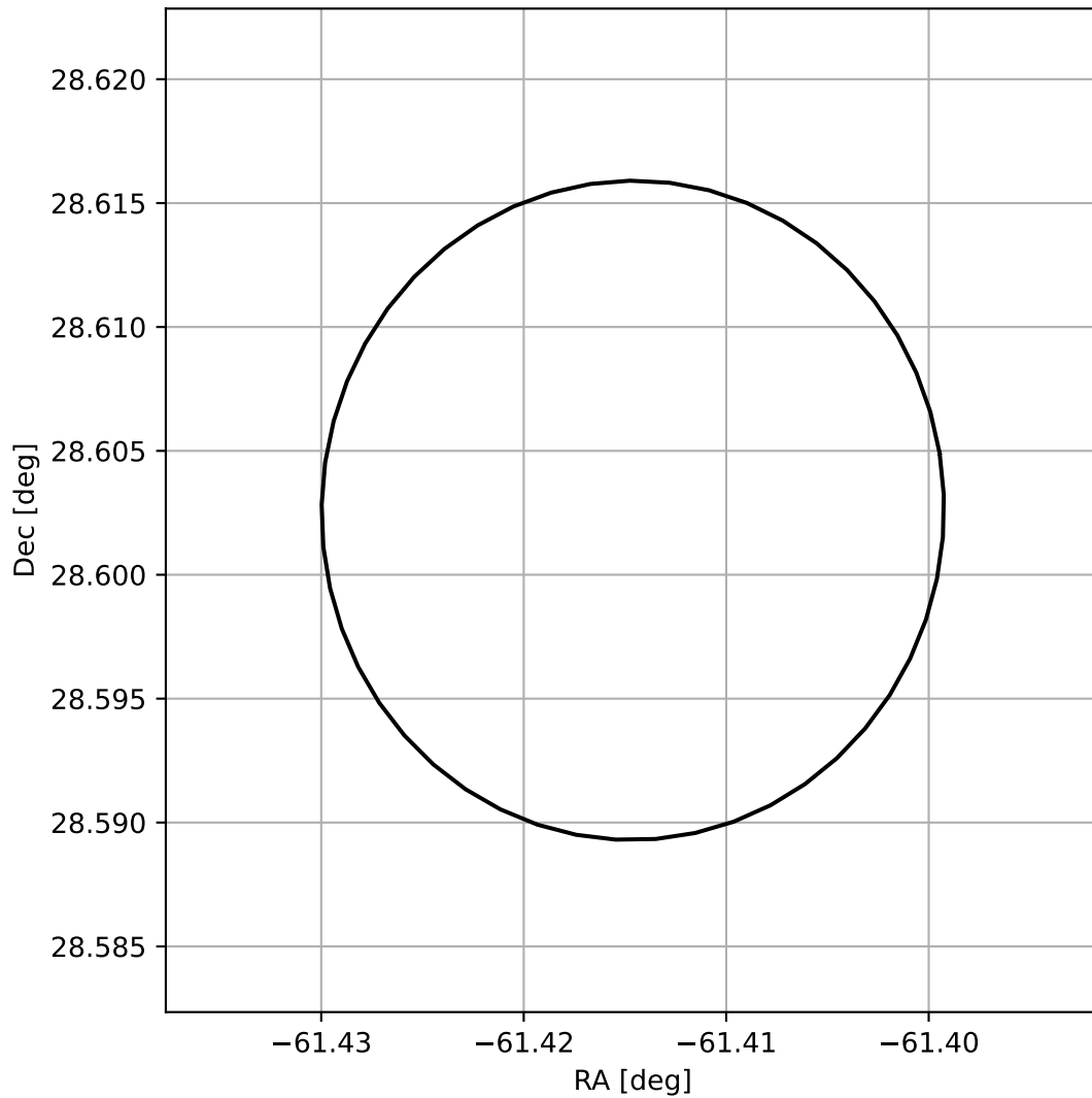
4FGL J1954.3+2836
