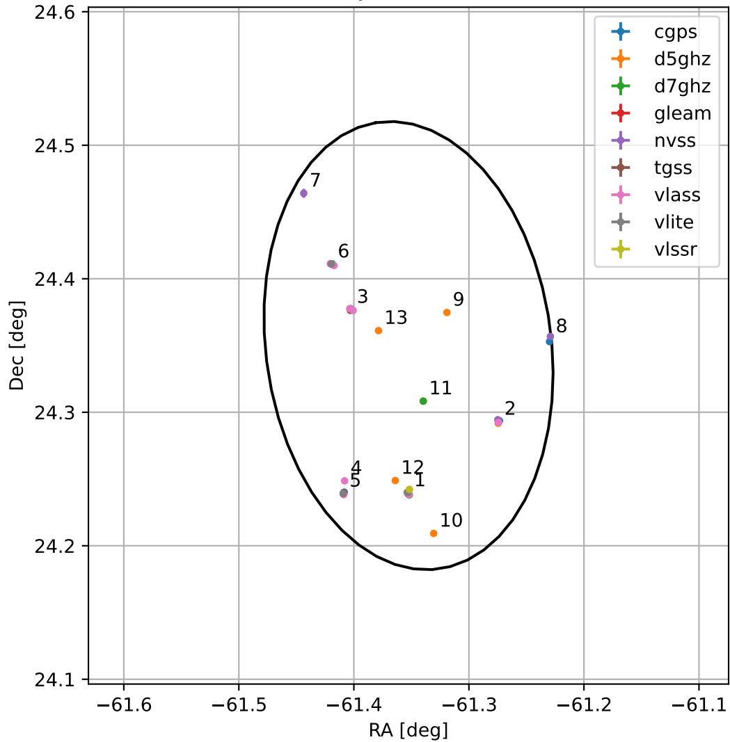
4FGL J1954.5+2420
