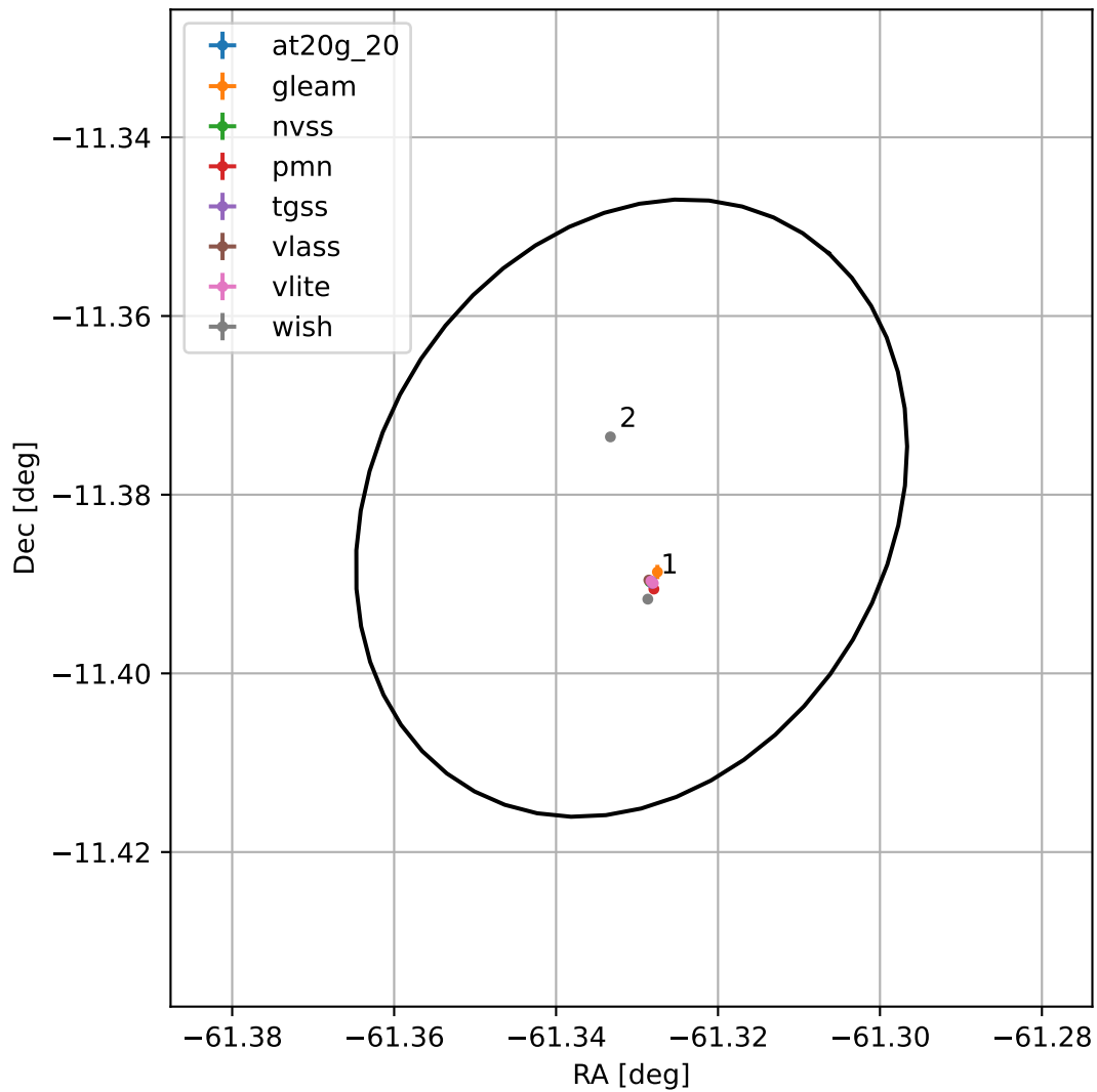
4FGL J1954.6-1122
