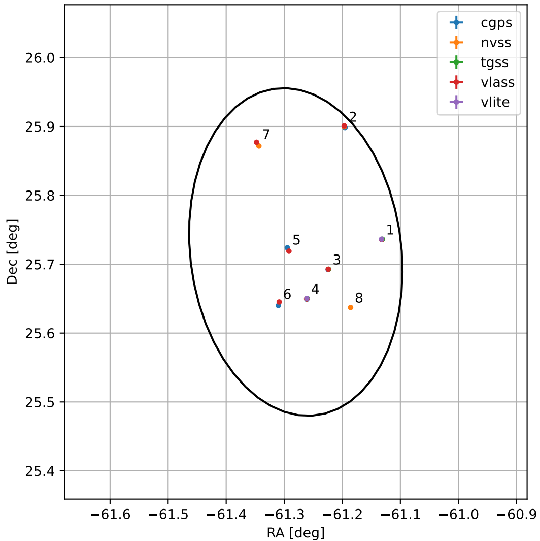
4FGL J1954.8+2543
