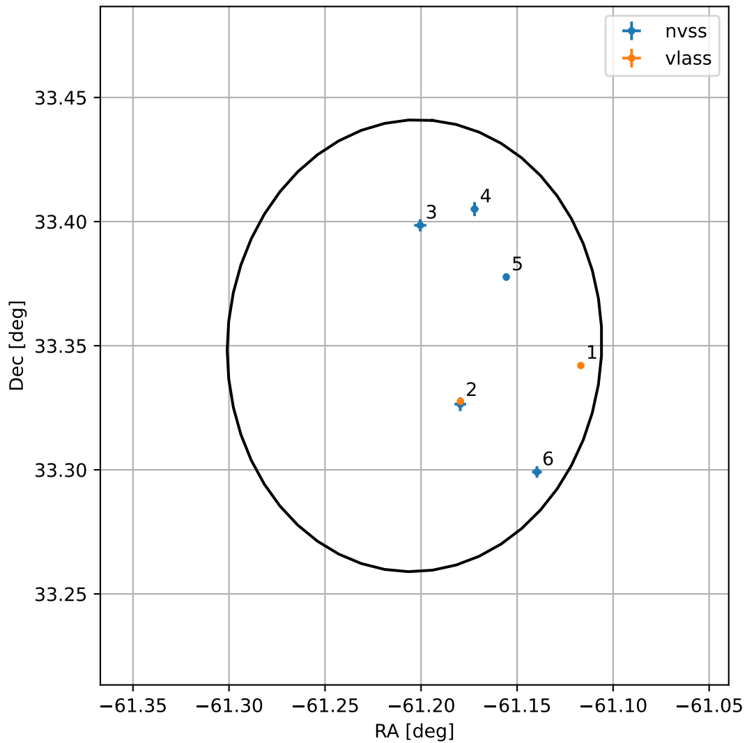
4FGL J1955.1+3321
